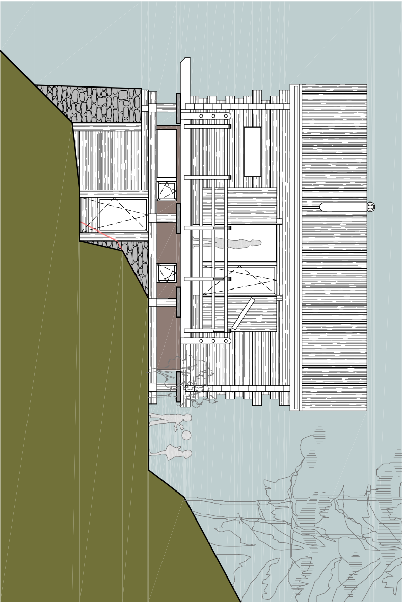
FACADE SUD
